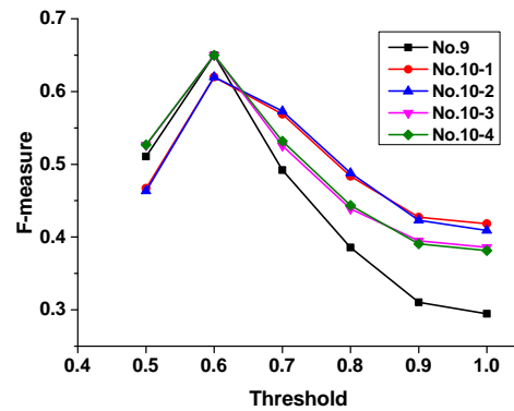
Figure 5: F-measures of xAST algorithm (No.9) and its variants (No.10-1,2,3,4)
